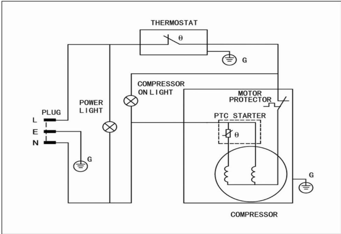
MWF9010/9013/9016 Daigram
