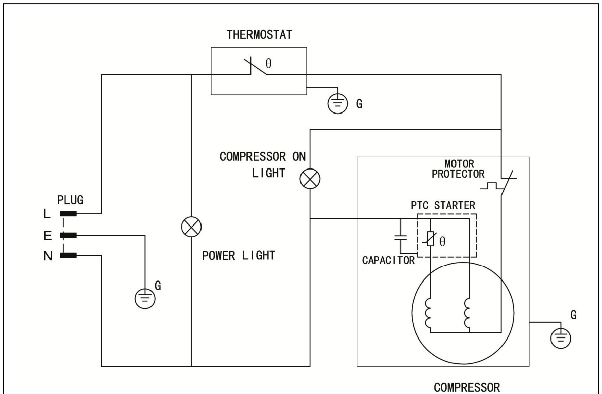
MWF9010/9013/9016 Daigram
