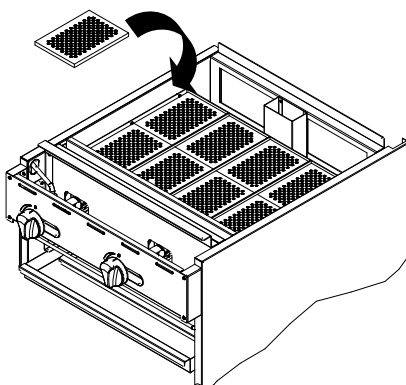
Step II: placing the ceramic plates
