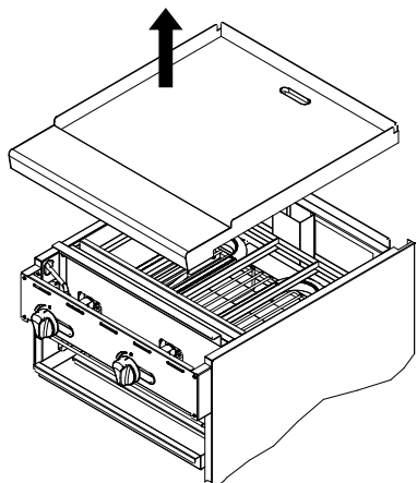
Step I: remove the griddle plate
